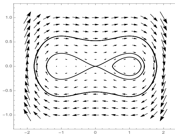
FIGURE 1. The vector field (X, Y) \mapsto (|Y|^{\frac{p}{p-1}-2} Y, |X|^{p-2} X - |X|^{q-2} X) and periodic trajectories corresponding to a = 1.35 (with positive X ) and a = 1.8 (with sign-changing X ) are shown for p = 2.5 and q = 3 . The zero-energy level is also shown.
