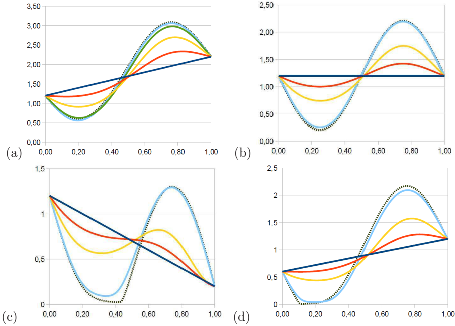
FIG. 1. Evolution towards the stationary state in the 1D case with sinusoidal potential (29). In each panel the initial datum is the straight line and the asymptotic solution is the dotted black curve. The other lines correspond to t = 0.012 , t = 0.024 , t = 0.048 , t = 0.1 . In panels (a) and (b) the two Dirichlet data are both supercritical (in particular, in panel (b) the asymptotic solution is u_0 - V(x_1) ). In panels (c) and (d), one of the data is subcritical (respectively, u_1 and u_0 ).
