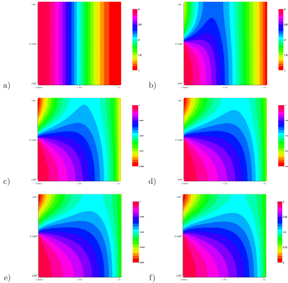
FIG. 7. Contours of the density u at six different instants: a) t = 0 (initial condition), b) t = 0.10 , c) t = 0.30 , d) t = 0.50 , e) t = 0.80 and f) t = 1.00 .
