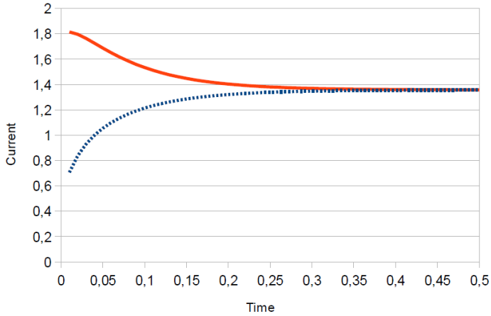
FIG. 4. Currents J_L (blue dotted line) and J_R (red continuous line) versus time under the action of the potential V(x_1) = e^{-(x_1 - .5)^2} and small gap between the boundary data in \Gamma_2 and \Gamma_4 .
