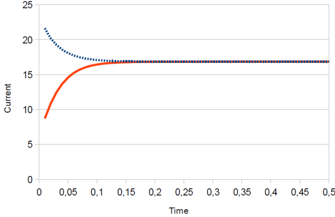
FIG. 5. Currents J_L (blue dotted line) and J_R (red continuous line) versus time under the action of the potential V(x_1) = e^{-(x_1-.5)^2} and wide gap between the boundary data in \Gamma_2 and \Gamma_4 .
